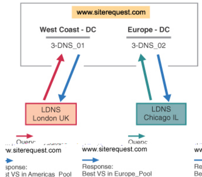
Figure 6.1 Topology load balancing in a globally-distributed network
